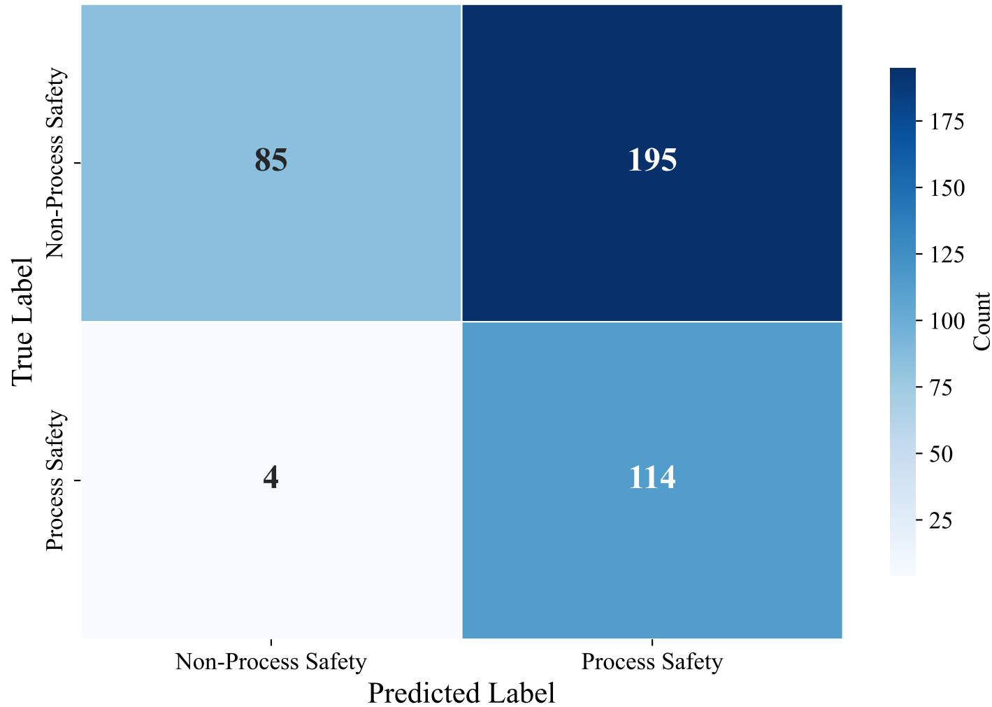
Confusion Matrix — DUTCH_MANUAL (upskyy/bge-m3-korean, Random_Forest_Optimized)
