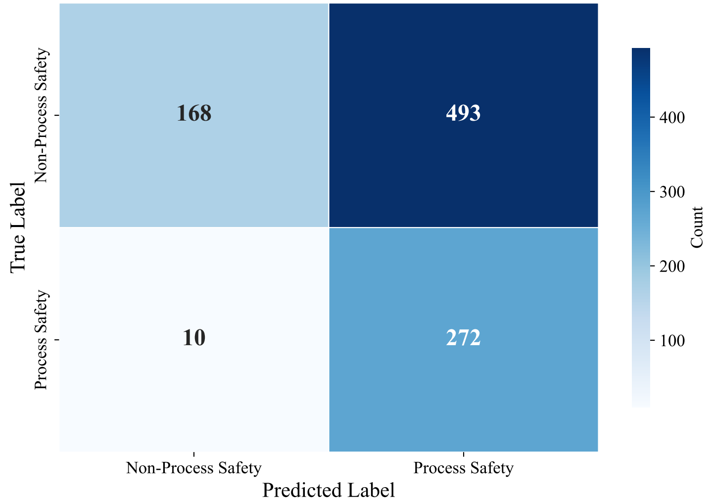
Confusion Matrix — ENGLISH_MANUAL (bert-base-multilingual-uncased, Random_Forest_Optimized)
