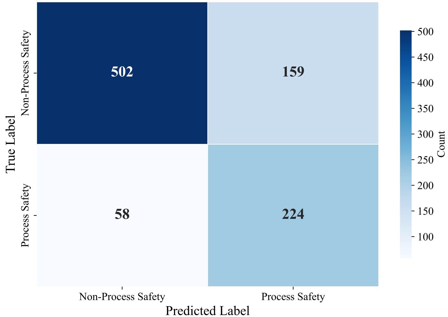
Confusion Matrix — ENGLISH_MANUAL (efederici/e5-base-multilingual-4096, LightGBM_Optimized)
