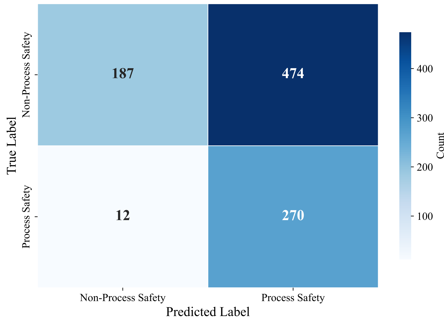
Confusion Matrix — ENGLISH_MANUAL (efederici/e5-base-multilingual-4096, Random_Forest_Optimized)
