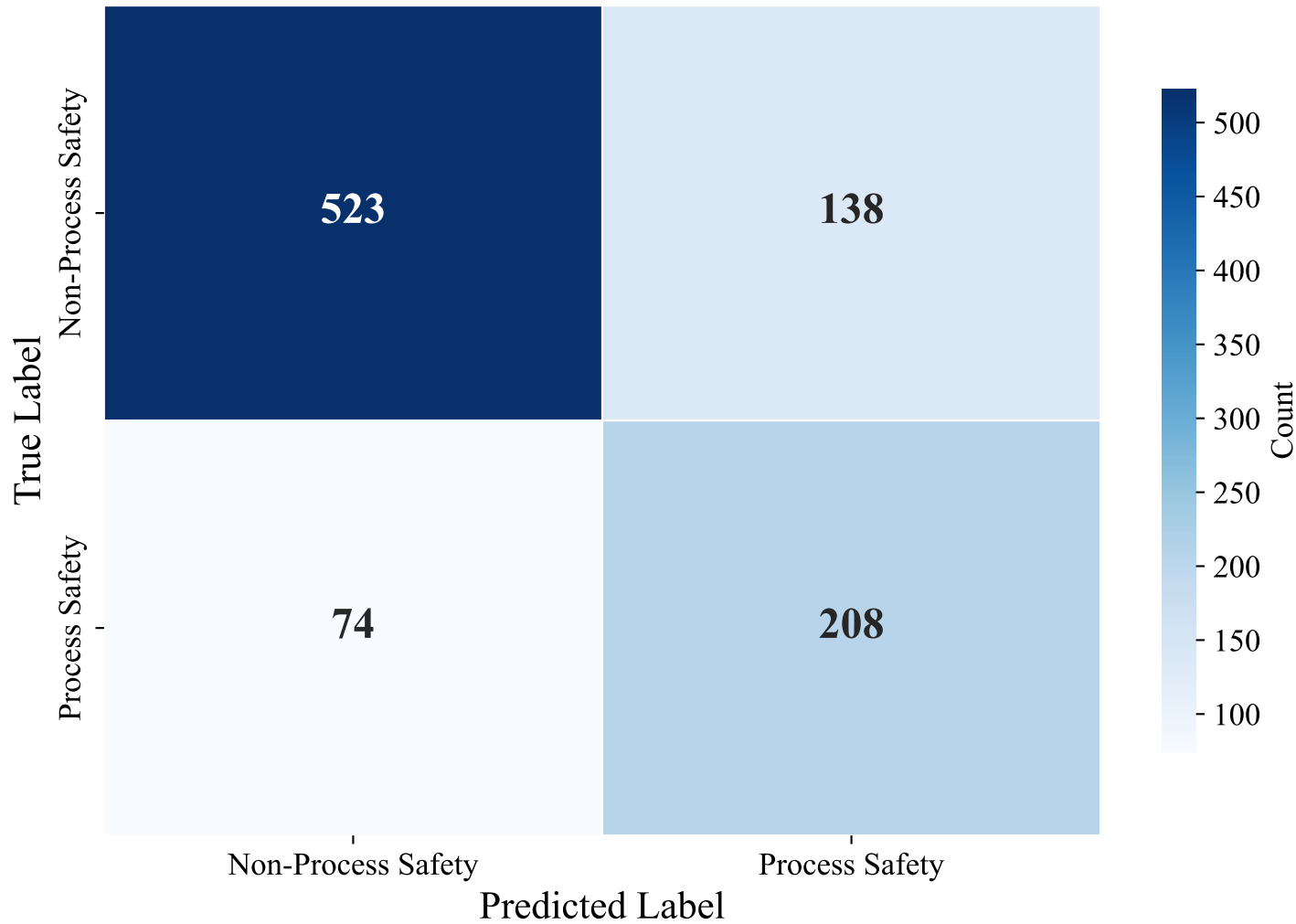
Confusion Matrix — ENGLISH_MANUAL (efederici/e5-base-multilingual-4096, SVM)
