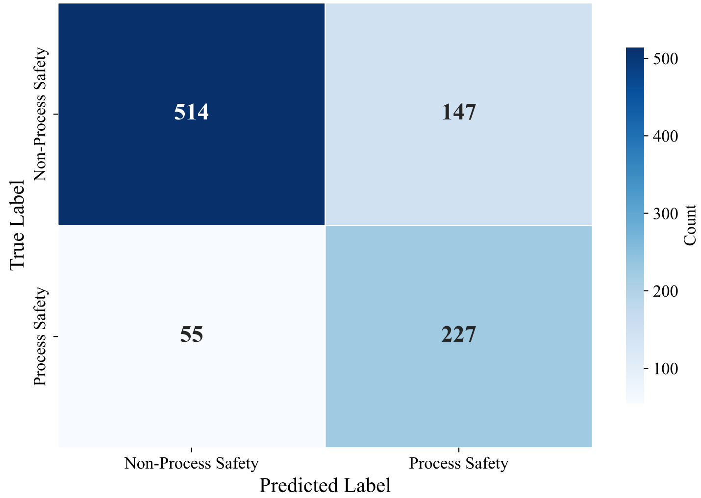
Confusion Matrix — ENGLISH_MANUAL (paraphrase-multilingual-mpnet-base-v2, LightGBM_Optimized)
