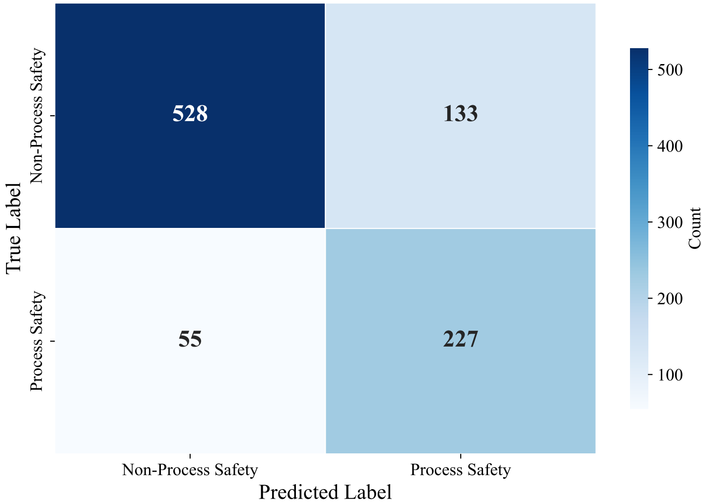
Confusion Matrix — ENGLISH_MANUAL (upskyy/bge-m3-korean, LightGBM)
