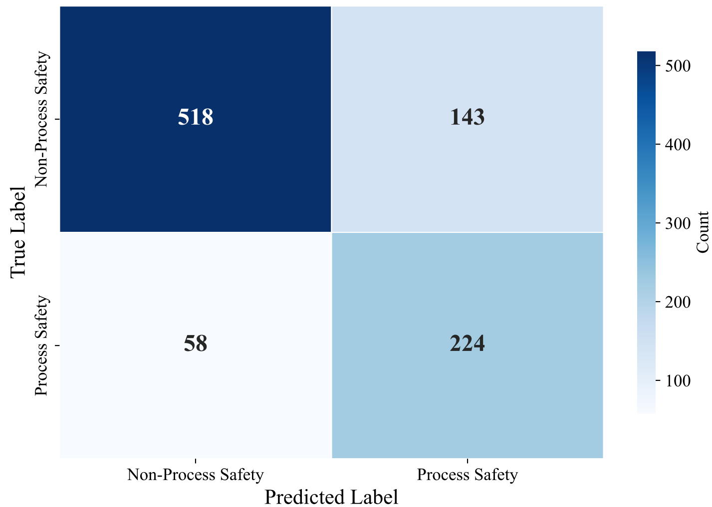
Confusion Matrix — ENGLISH_MANUAL (upskyy/bge-m3-korean, XGBoost)
