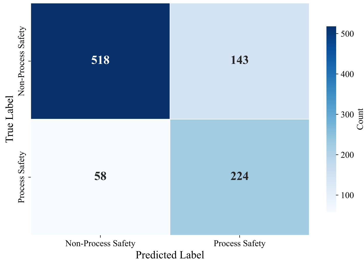
Confusion Matrix — ENGLISH_MANUAL (upskyy/bge-m3-korean, XGBoost_Optimized)
