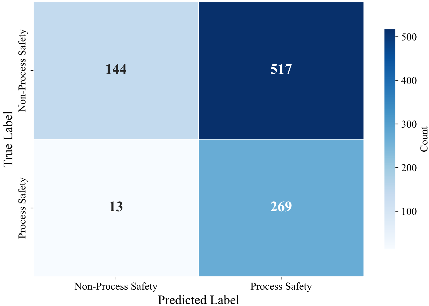
Confusion Matrix — ENGLISH_MANUAL (xlm-roberta-base, Random_Forest_Optimized)
