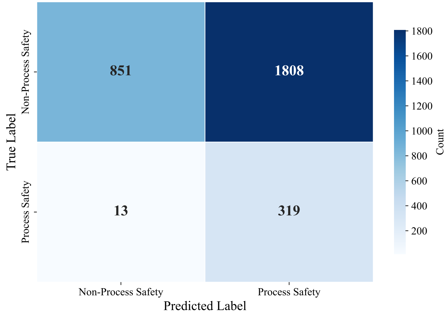
Confusion Matrix — GERMAN_MANUAL (bert-base-multilingual-uncased, Random_Forest_Optimized)
