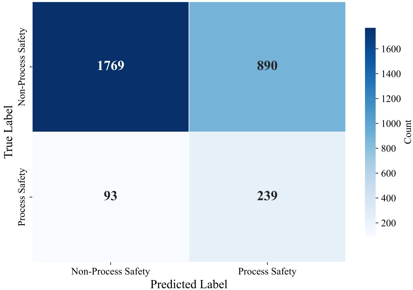
Confusion Matrix — GERMAN_MANUAL (efederici/e5-base-multilingual-4096, Random_Forest)
