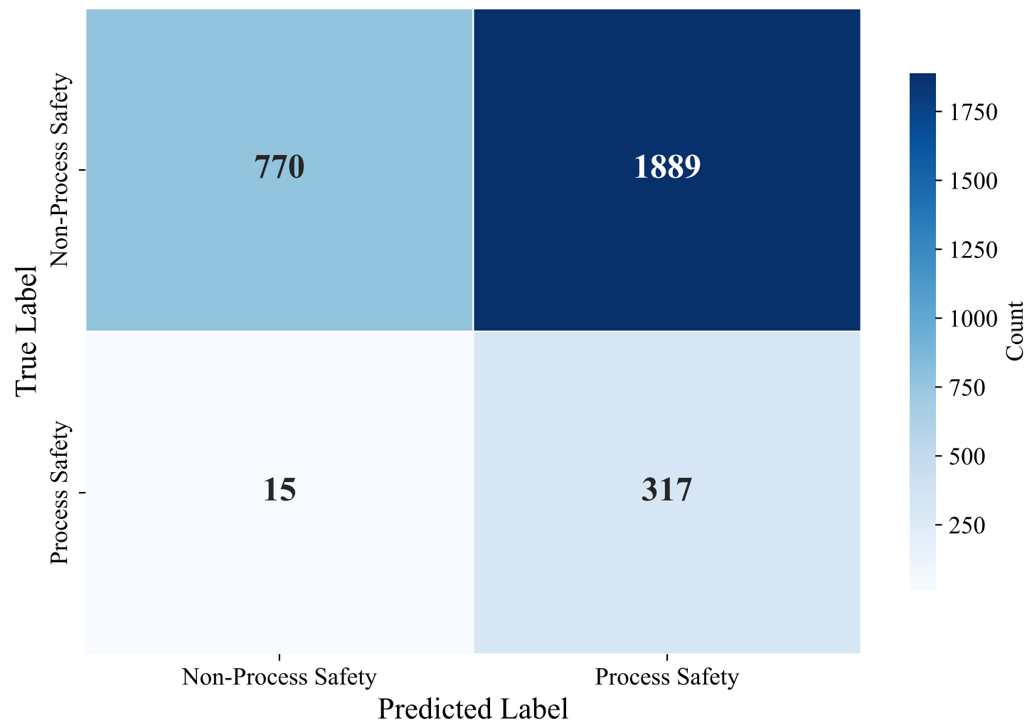
Confusion Matrix — GERMAN_MANUAL (efederici/e5-base-multilingual-4096, Random_Forest_Optimized)
