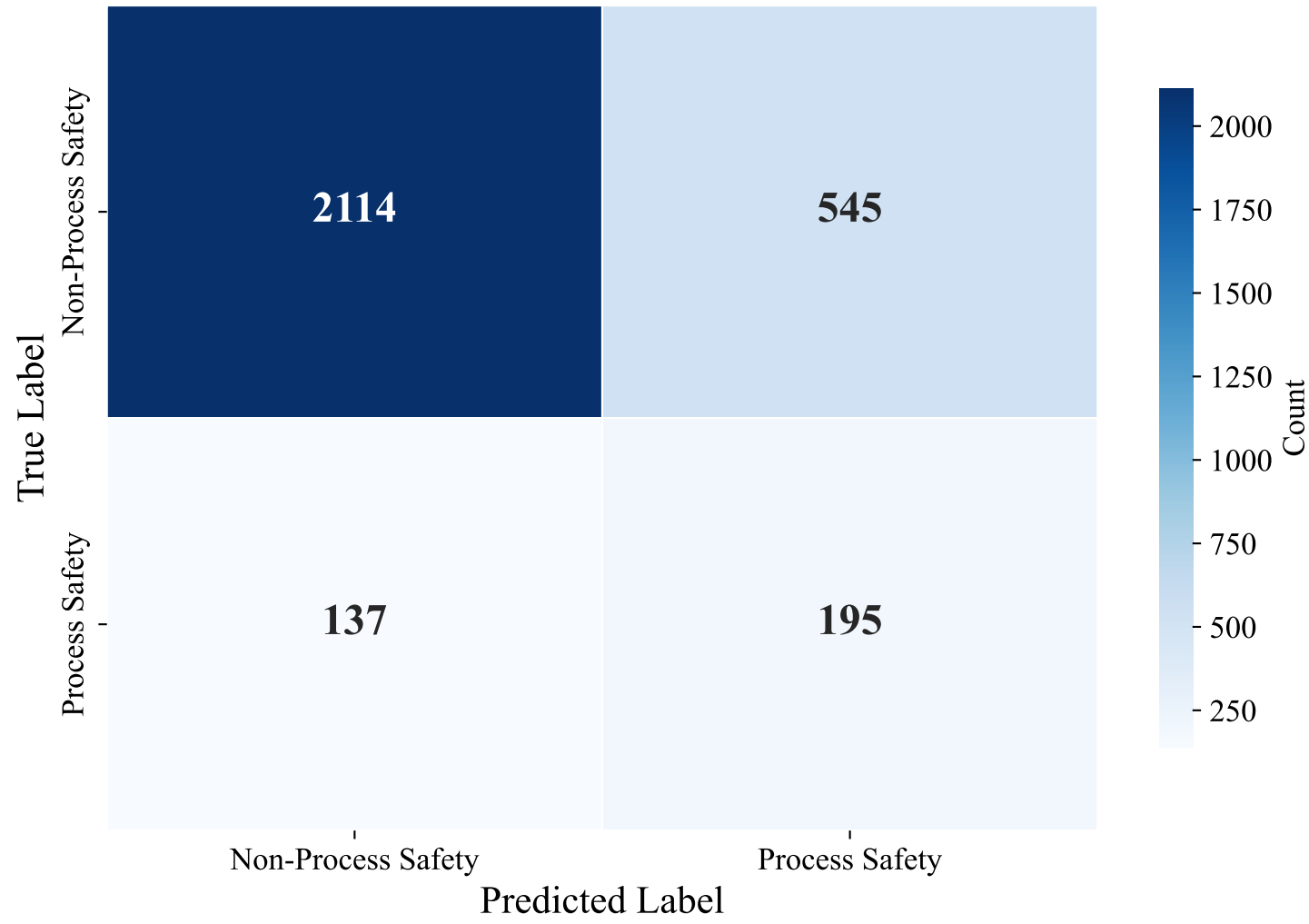
Confusion Matrix — GERMAN_MANUAL (paraphrase-multilingual-MiniLM-L12-v2, LightGBM_Optimized)
