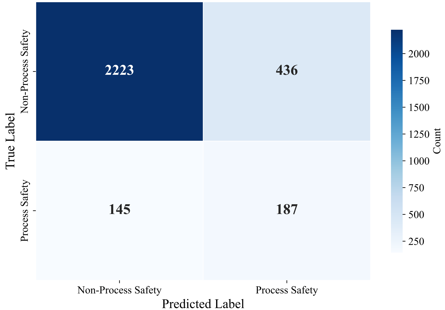
Confusion Matrix — GERMAN_MANUAL (paraphrase-multilingual-MiniLM-L12-v2, XGBoost_Optimized)
