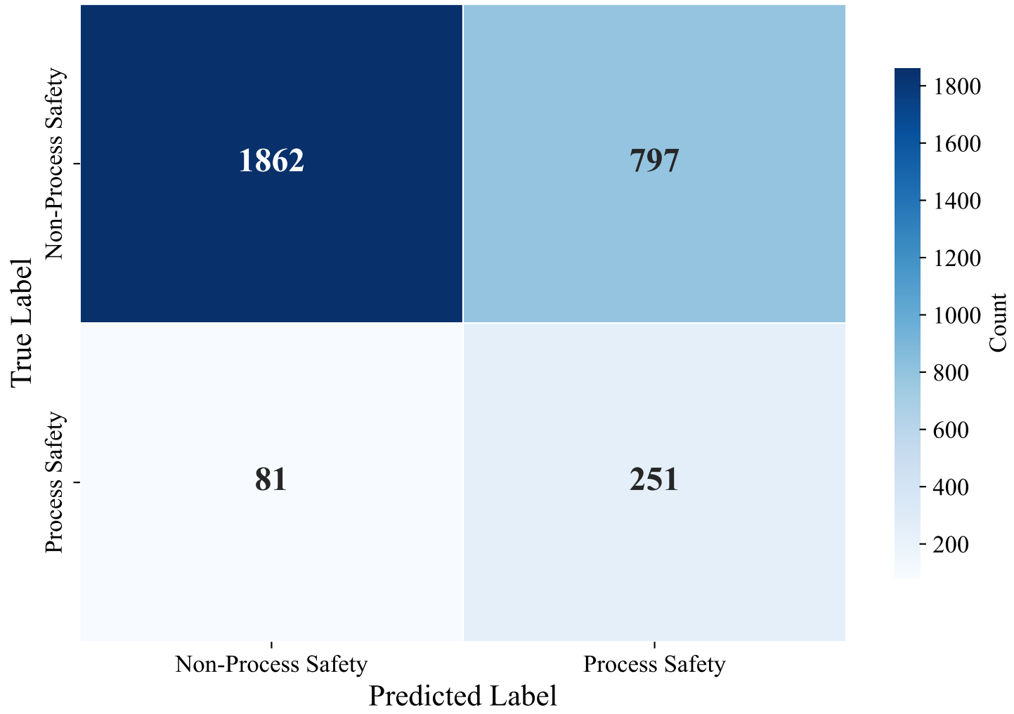
Confusion Matrix — GERMAN_MANUAL (upskyy/bge-m3-korean, Random_Forest)
