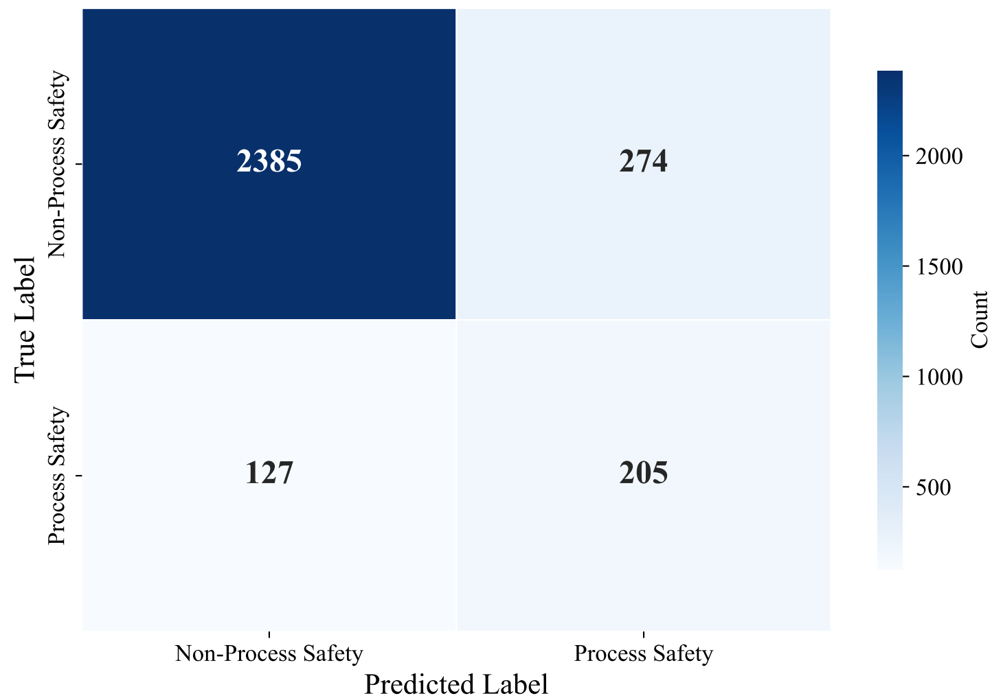
Confusion Matrix — GERMAN_MANUAL (upskyy/bge-m3-korean, XGBoost)
