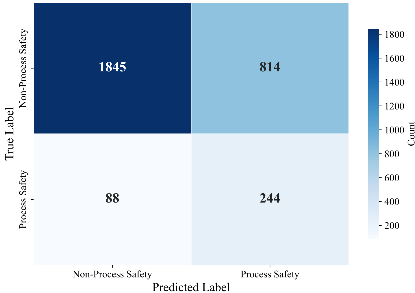
Confusion Matrix — GERMAN_MANUAL (xlm-roberta-base, Random_Forest)
