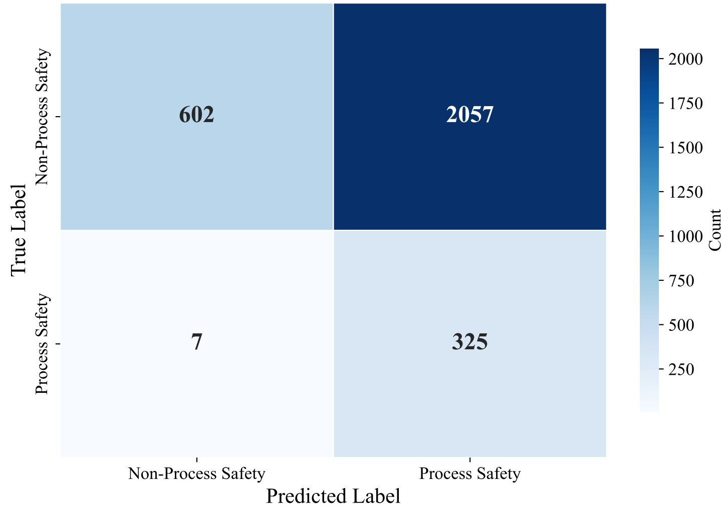
Confusion Matrix — GERMAN_MANUAL (xlm-roberta-base, Random_Forest_Optimized)
