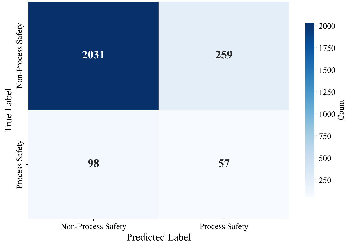
Confusion Matrix — SWEDISH_MANUAL (bert-base-multilingual-uncased, Voting_Ensemble)
