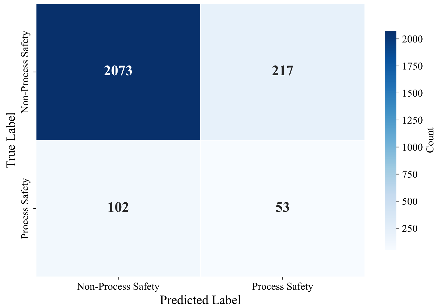
Confusion Matrix — SWEDISH_MANUAL (bert-base-multilingual-uncased, XGBoost_Optimized)
