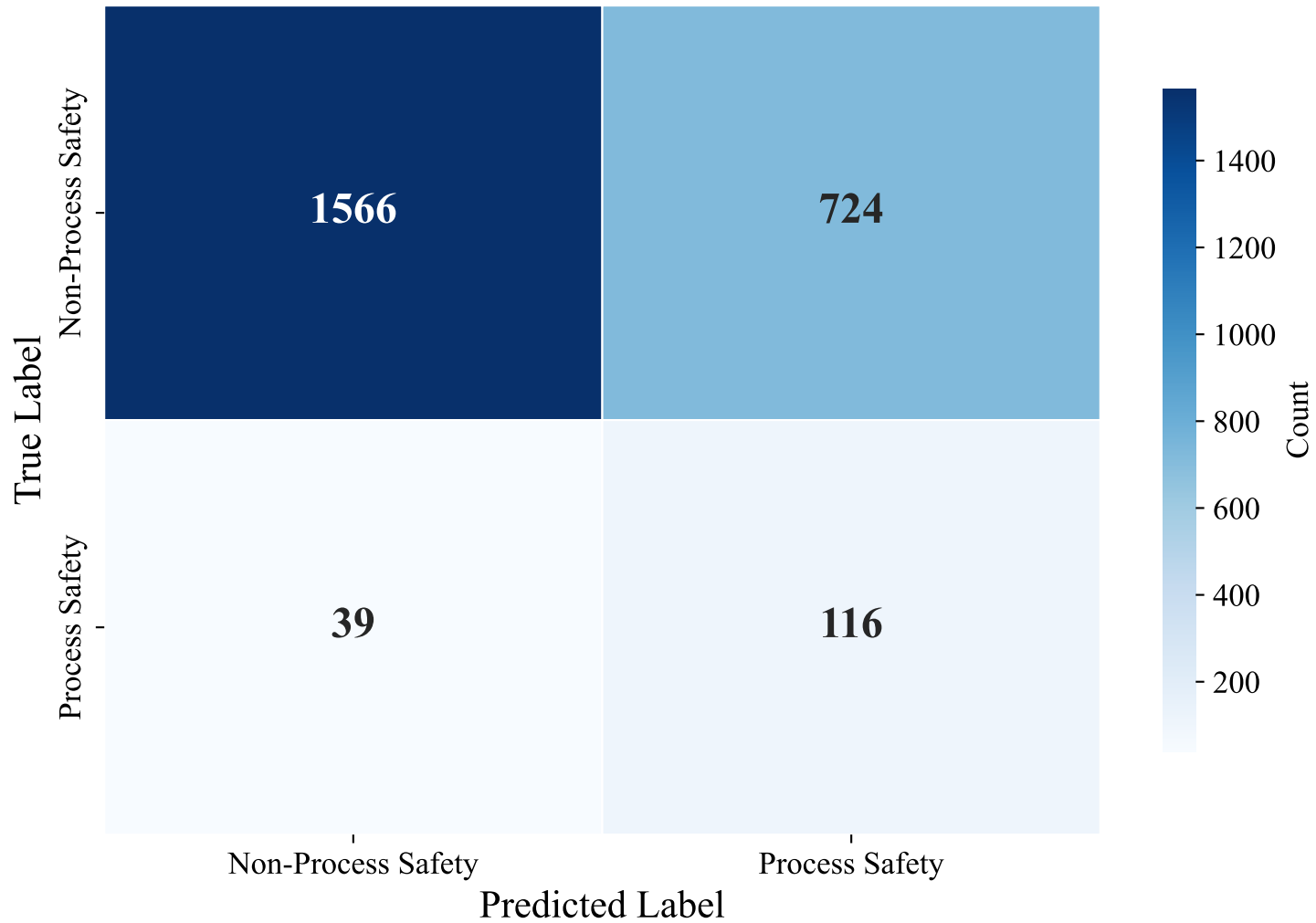
Confusion Matrix — SWEDISH_MANUAL (efederici/e5-base-multilingual-4096, Random_Forest)
