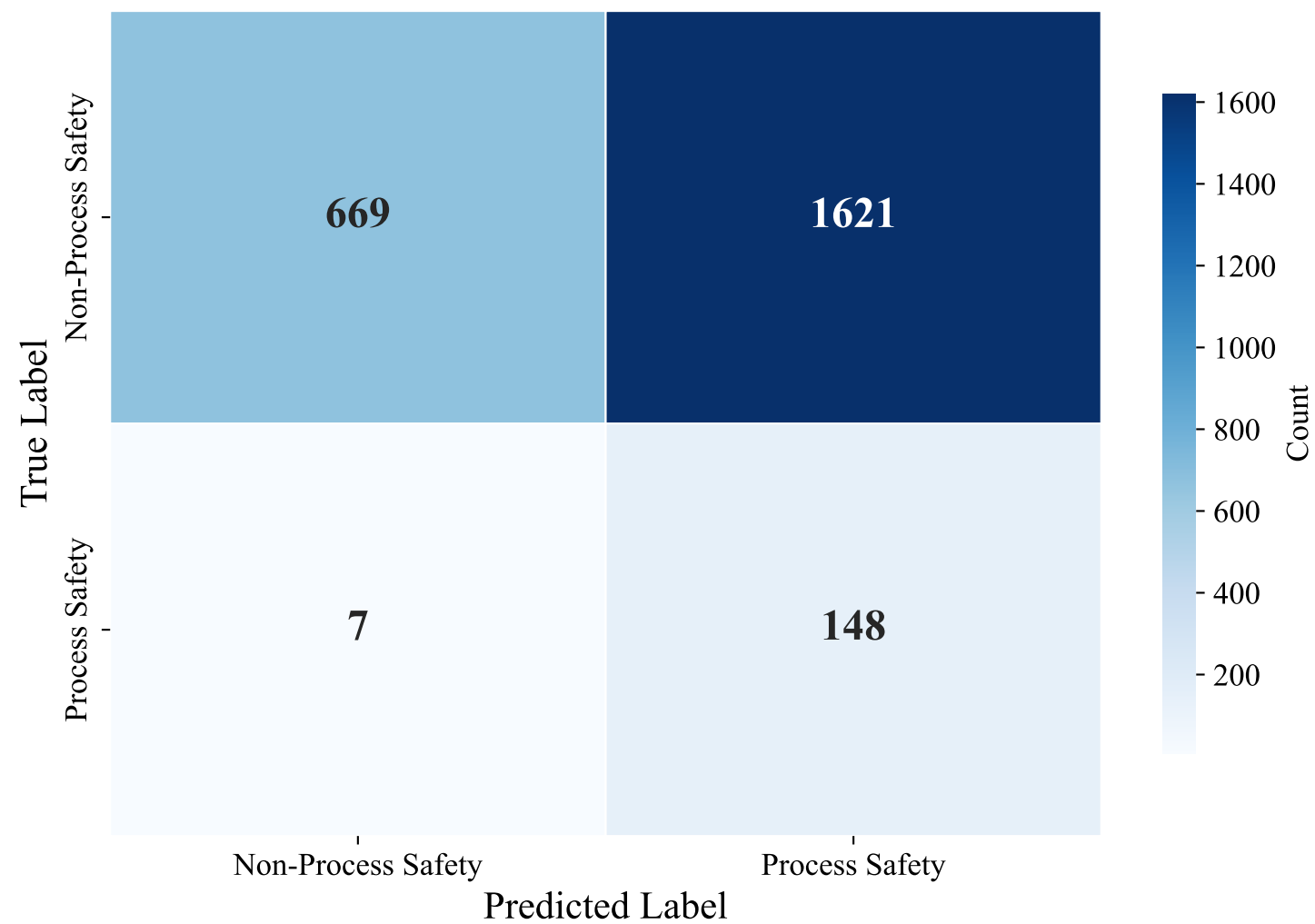
Confusion Matrix — SWEDISH_MANUAL (efederici/e5-base-multilingual-4096, Random_Forest_Optimized)
