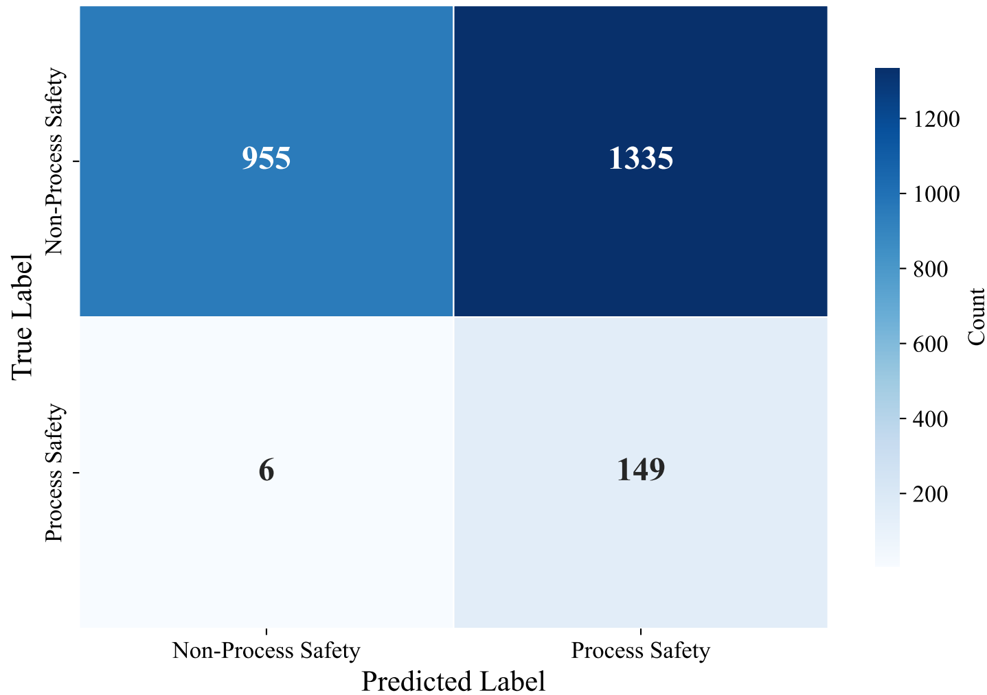
Confusion Matrix — SWEDISH_MANUAL (intfloat/multilingual-e5-large-instruct, Random_Forest_Optimized)
