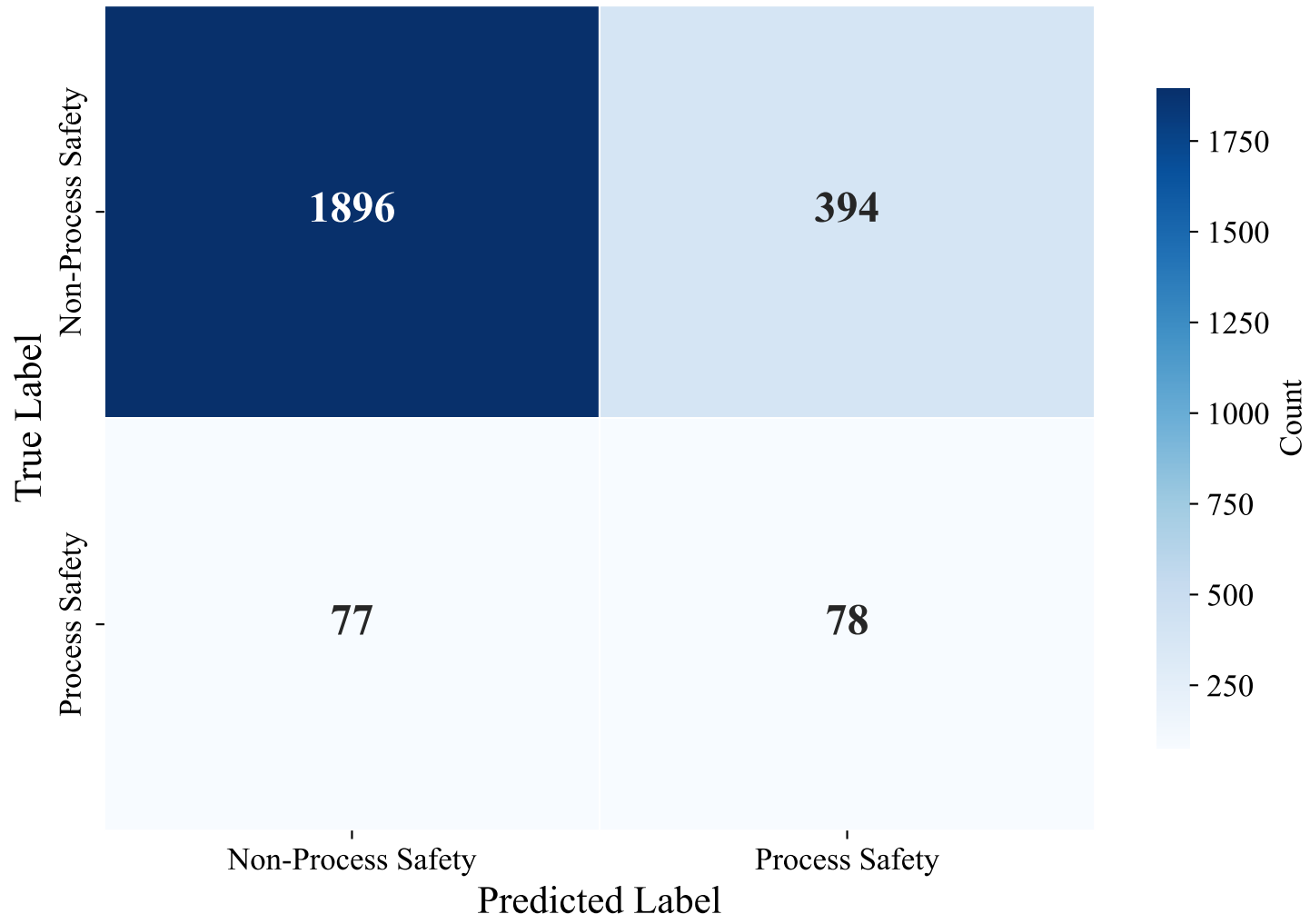
Confusion Matrix — SWEDISH_MANUAL (intfloat/multilingual-e5-large-instruct, SVM)
