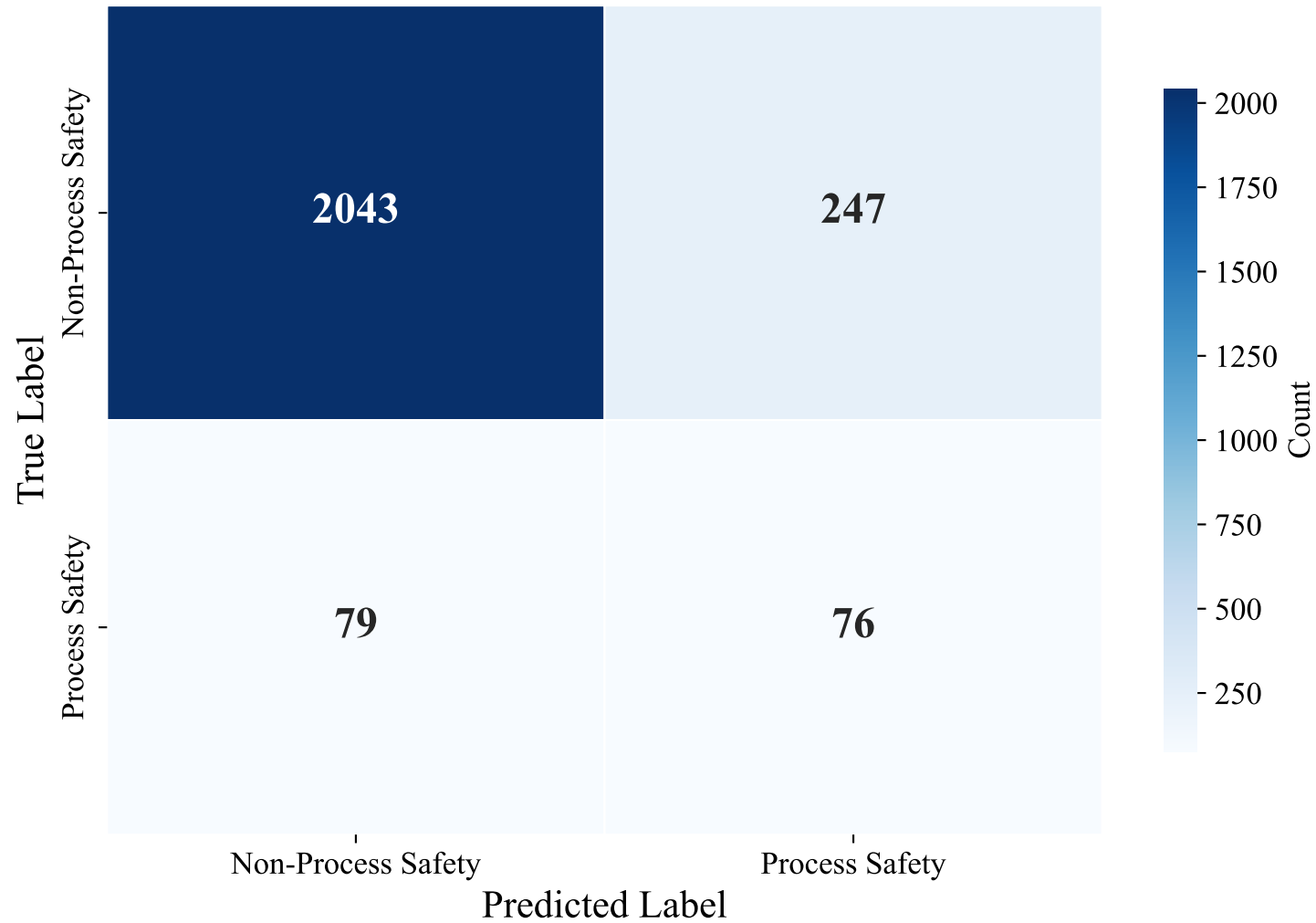
Confusion Matrix — SWEDISH_MANUAL (intfloat/multilingual-e5-large-instruct, Voting_Ensemble)
