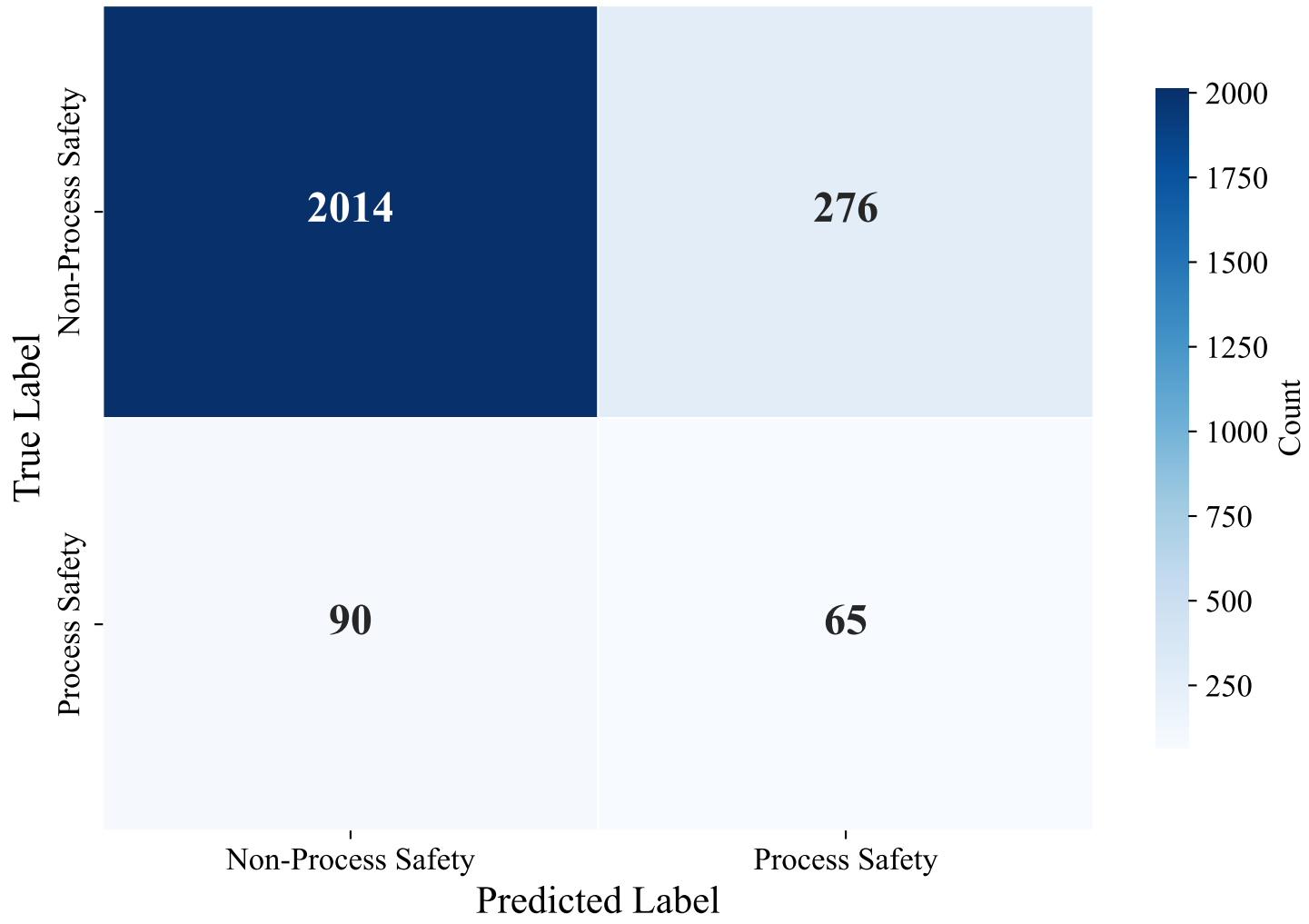
Confusion Matrix — SWEDISH_MANUAL (paraphrase-multilingual-MiniLM-L12-v2, LightGBM)
