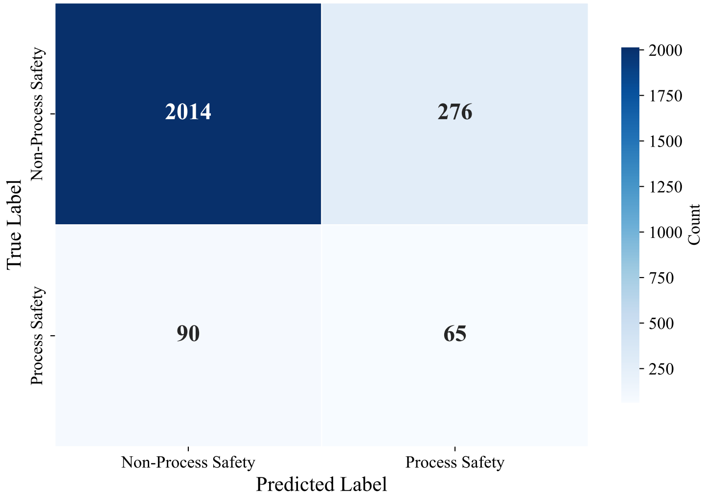
Confusion Matrix — SWEDISH_MANUAL (paraphrase-multilingual-MiniLM-L12-v2, LightGBM_Optimized)
