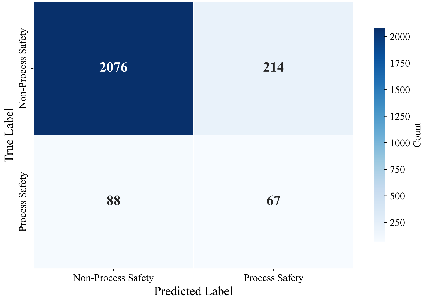
Confusion Matrix — SWEDISH_MANUAL (snowflake-arctic-embed-l-v2.0, LightGBM)
