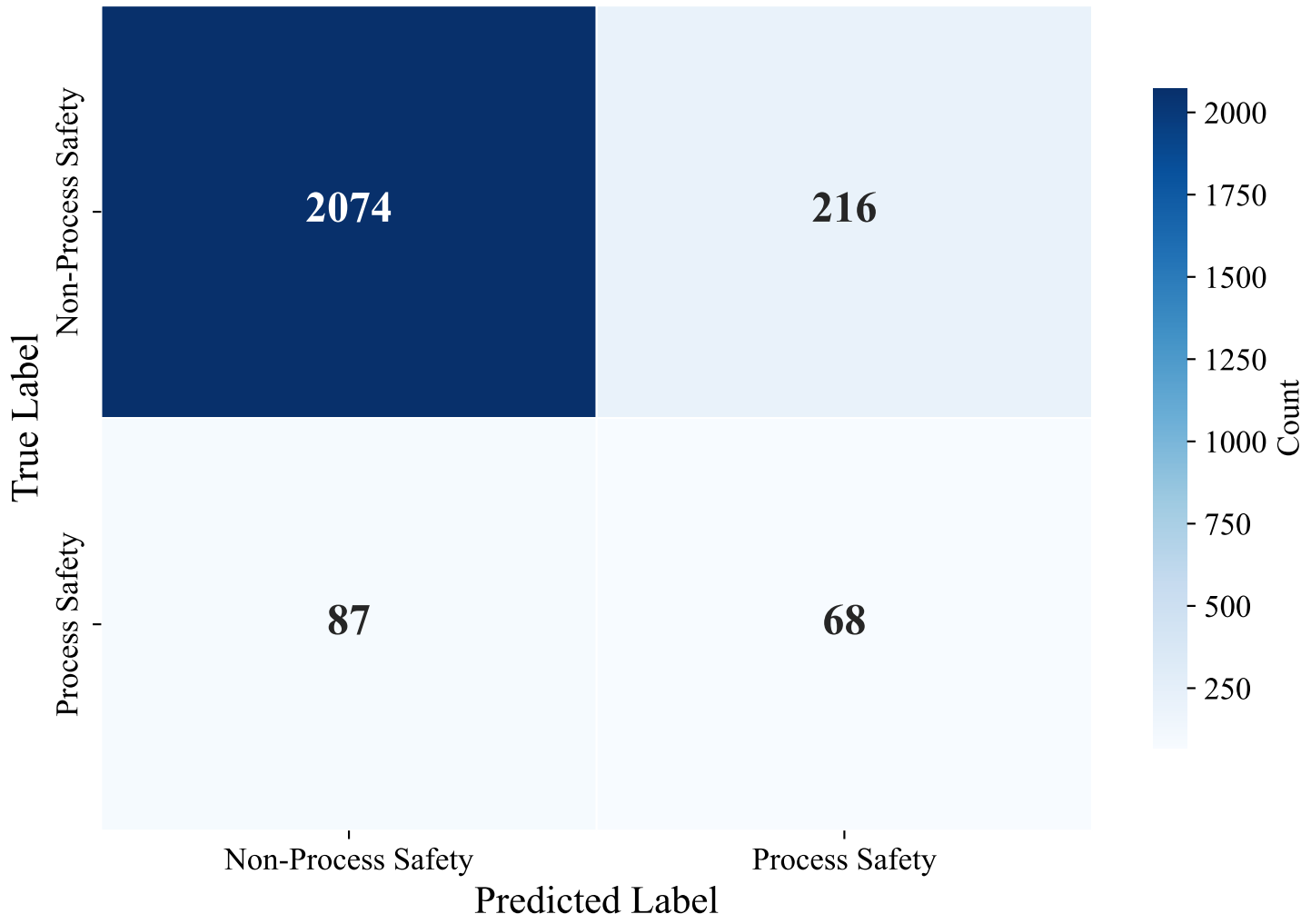
Confusion Matrix — SWEDISH_MANUAL (xlm-roberta-base, XGBoost)
