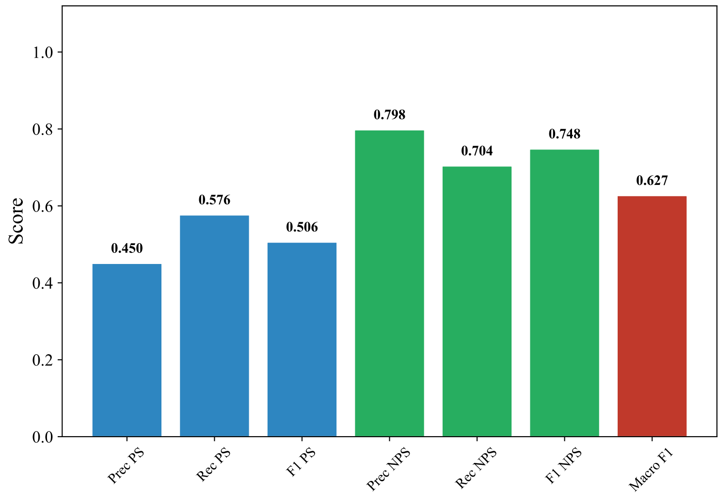
Classification Metrics — DUTCH_MANUAL (bert-base-multilingual-uncased, SVM)
