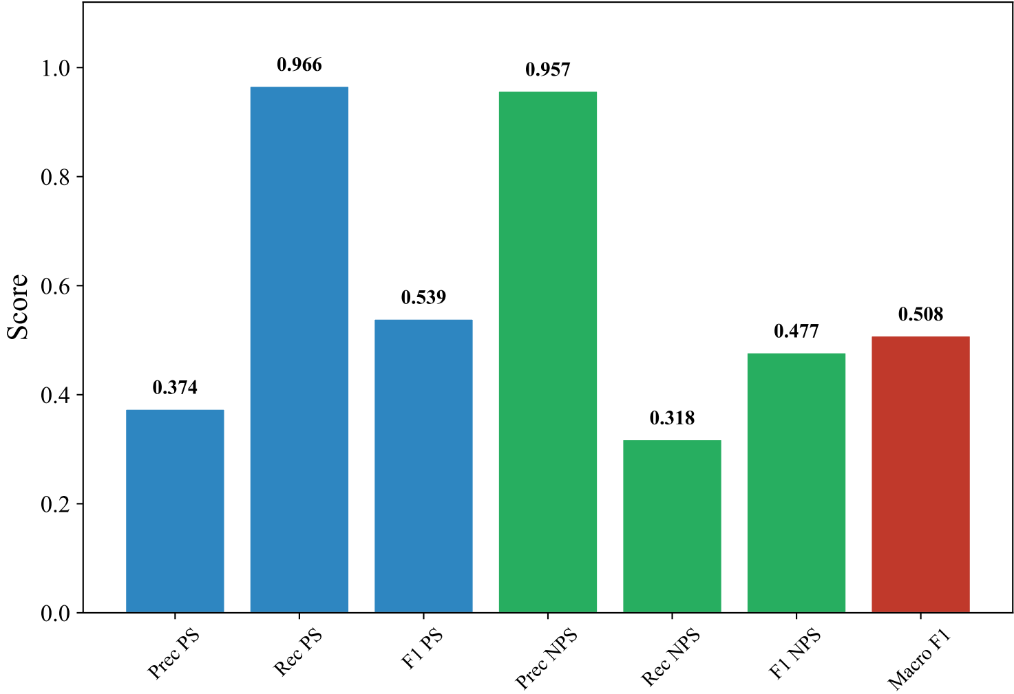
Classification Metrics — DUTCH_MANUAL (efederici/e5-base-multilingual-4096, Random_Forest_Optimized)
