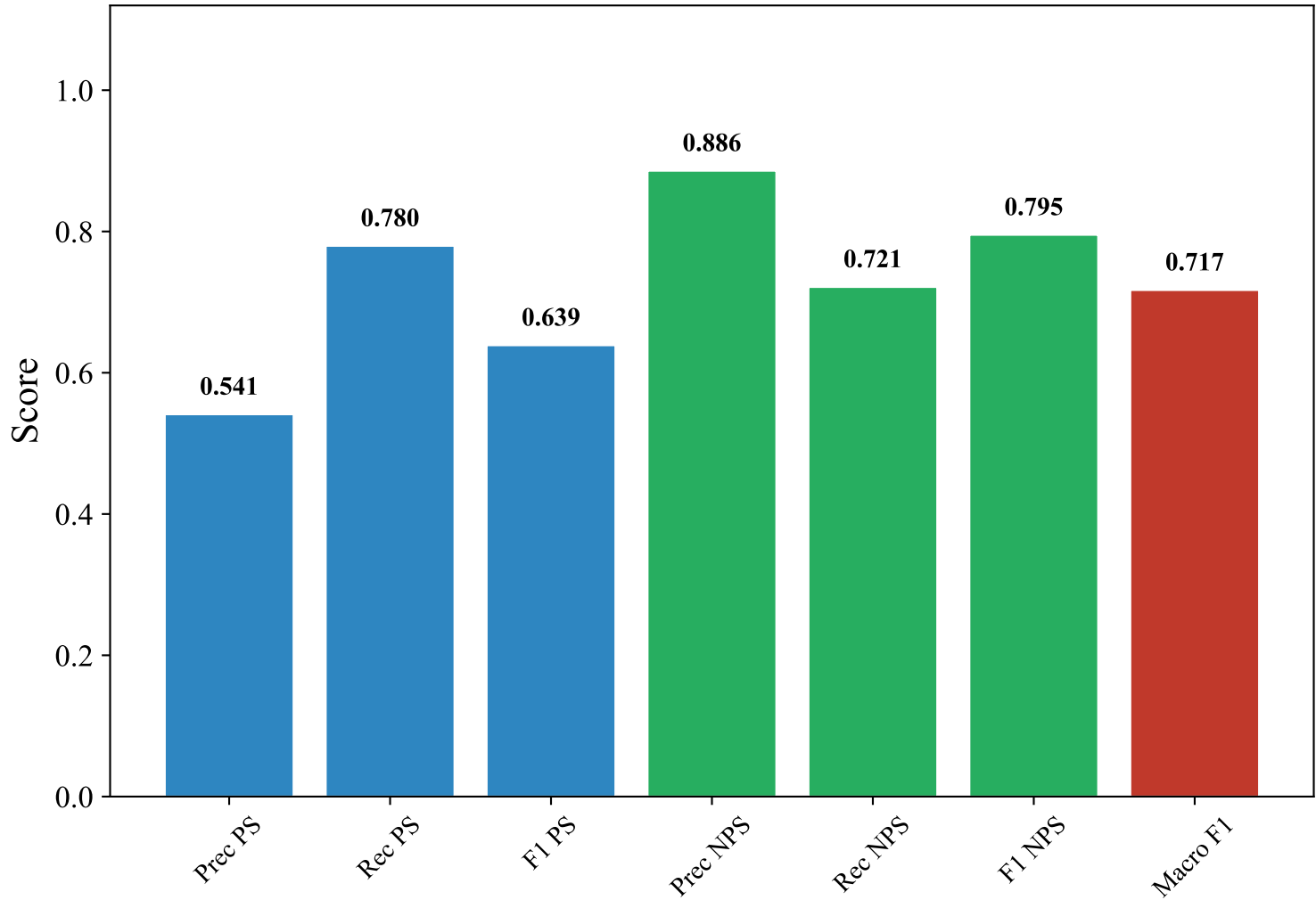
Classification Metrics — DUTCH_MANUAL (intfloat/multilingual-e5-large-instruct, XGBoost)
