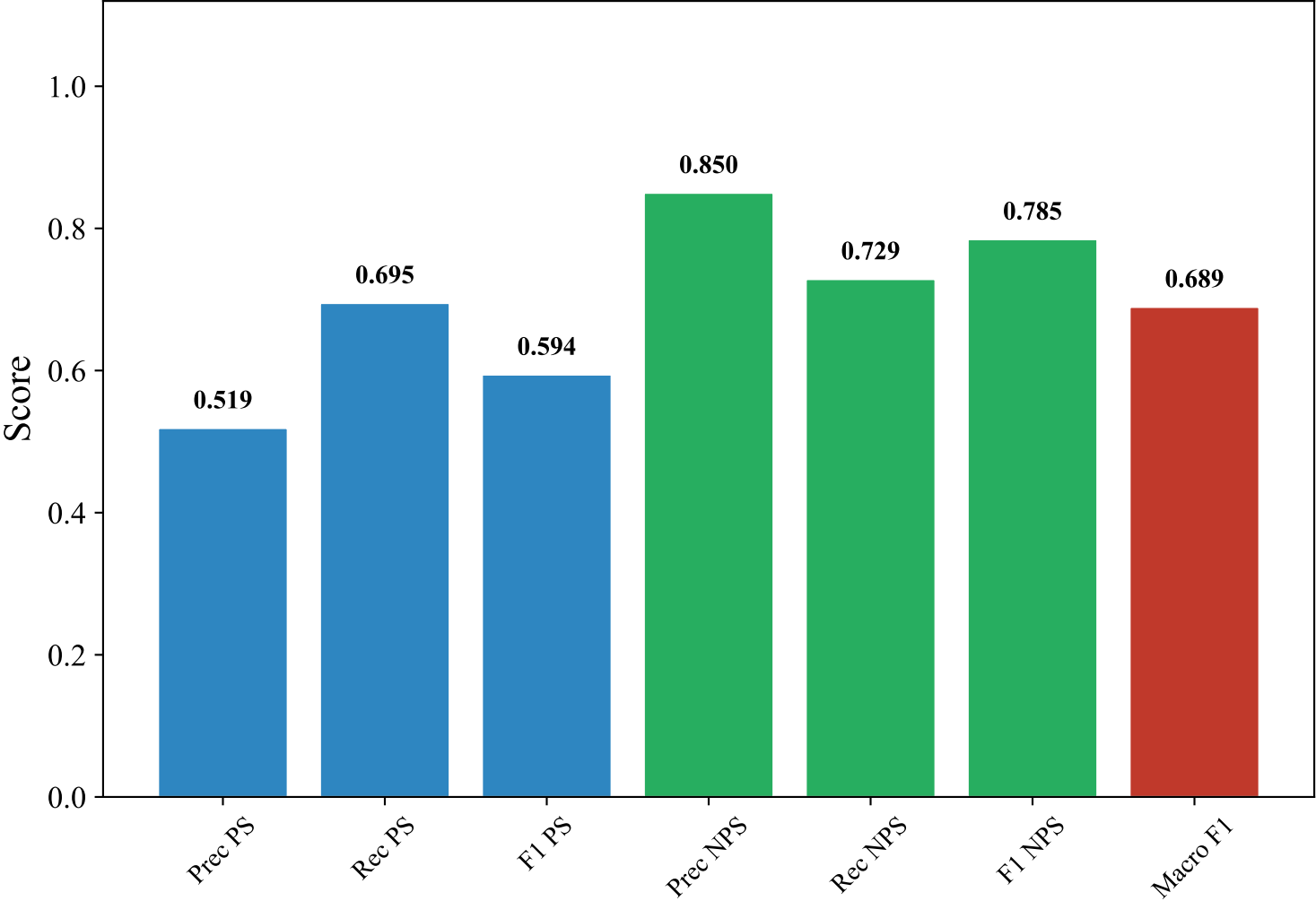
Classification Metrics — DUTCH_MANUAL (paraphrase-multilingual-MiniLM-L12-v2, LightGBM_Optimized)
