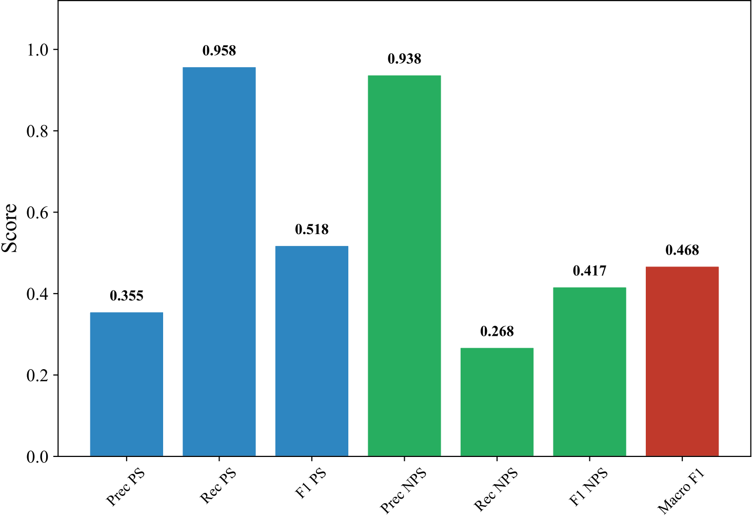
Classification Metrics — DUTCH_MANUAL (paraphrase-multilingual-mpnet-base-v2, Random_Forest_Optimized)
