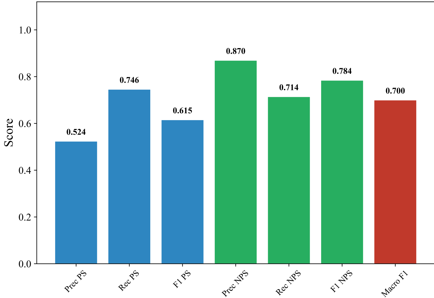
Classification Metrics — DUTCH_MANUAL (paraphrase-multilingual-mpnet-base-v2, XGBoost_Optimized)
