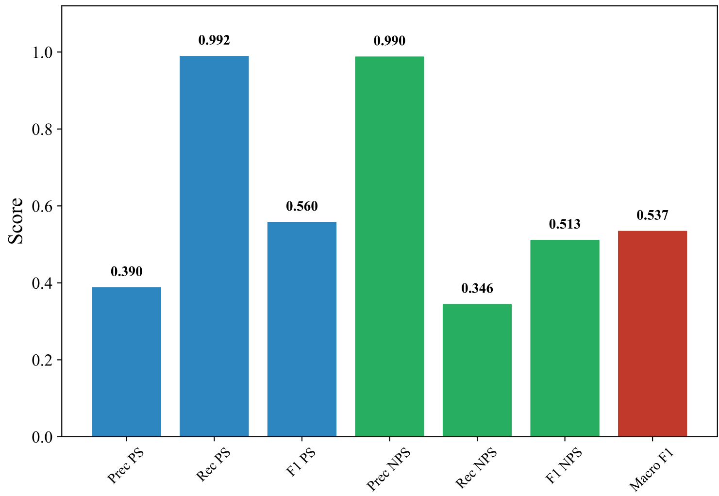
Classification Metrics — DUTCH_MANUAL (snowflake-arctic-embed-l-v2.0, Random_Forest_Optimized)
