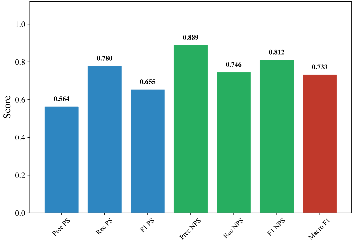
Classification Metrics — DUTCH_MANUAL (upskyy/bge-m3-korean, LightGBM_Optimized)
