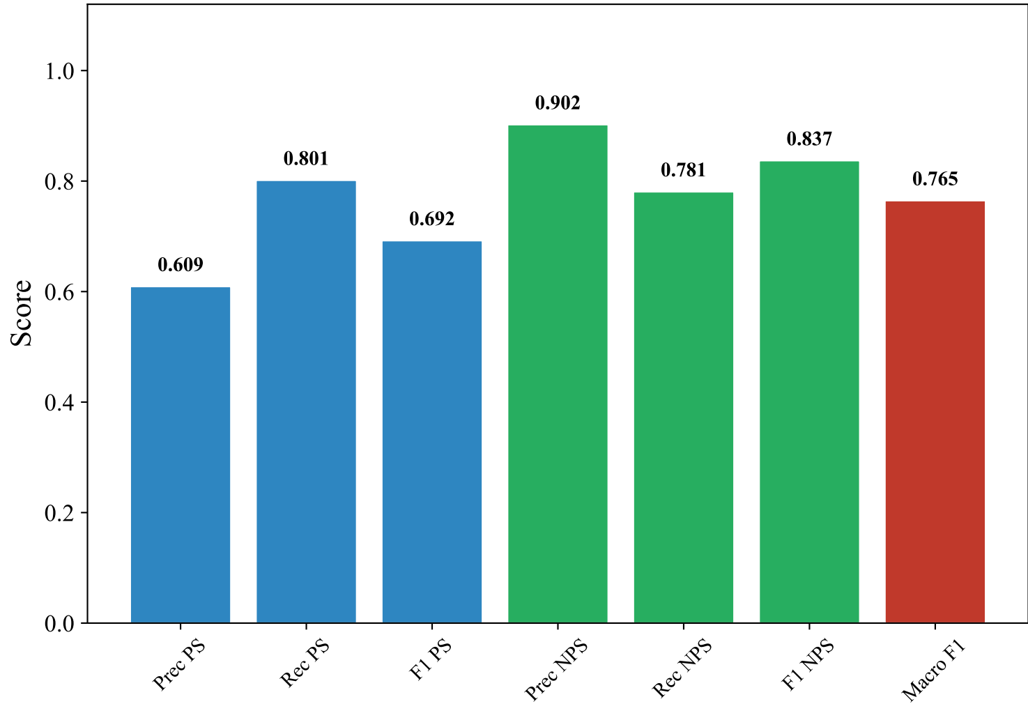
Classification Metrics — ENGLISH_MANUAL (paraphrase-multilingual-MiniLM-L12-v2, LightGBM)
