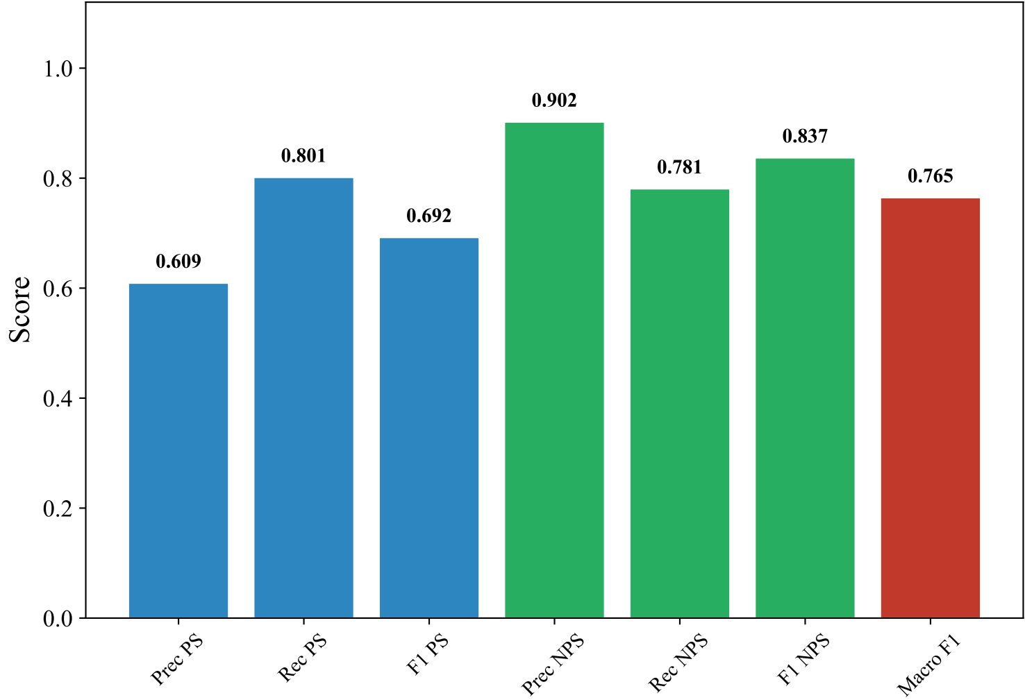
Classification Metrics — ENGLISH_MANUAL (paraphrase-multilingual-MiniLM-L12-v2, LightGBM_Optimized)
