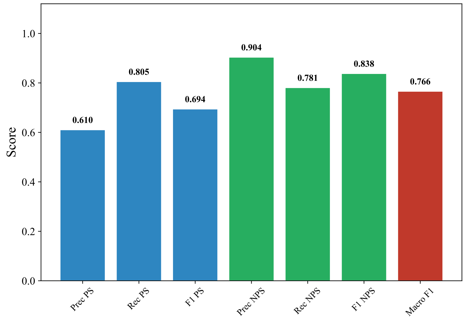
Classification Metrics — ENGLISH_MANUAL (paraphrase-multilingual-MiniLM-L12-v2, XGBoost)
