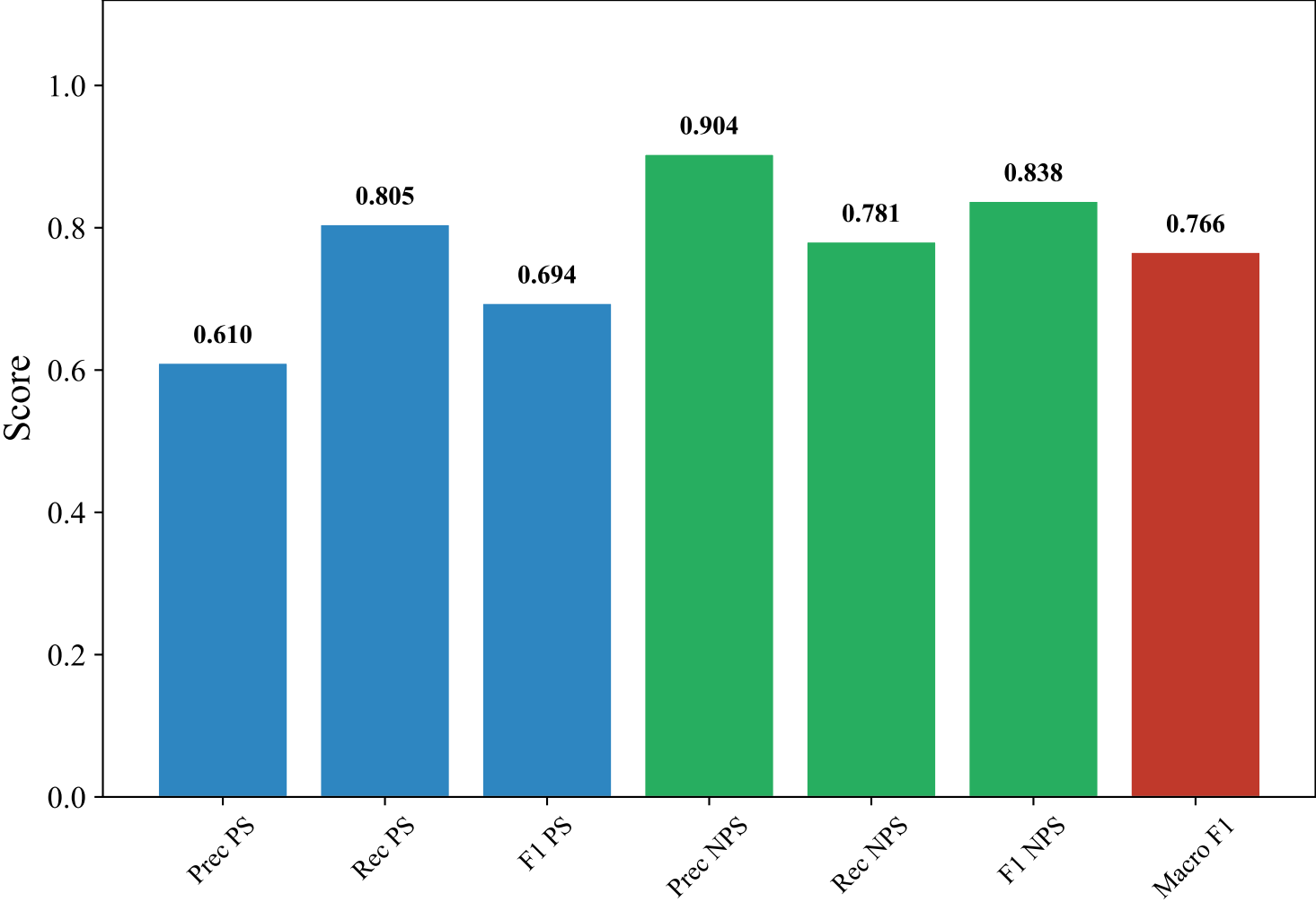
Classification Metrics — ENGLISH_MANUAL (paraphrase-multilingual-MiniLM-L12-v2, XGBoost_Optimized)
