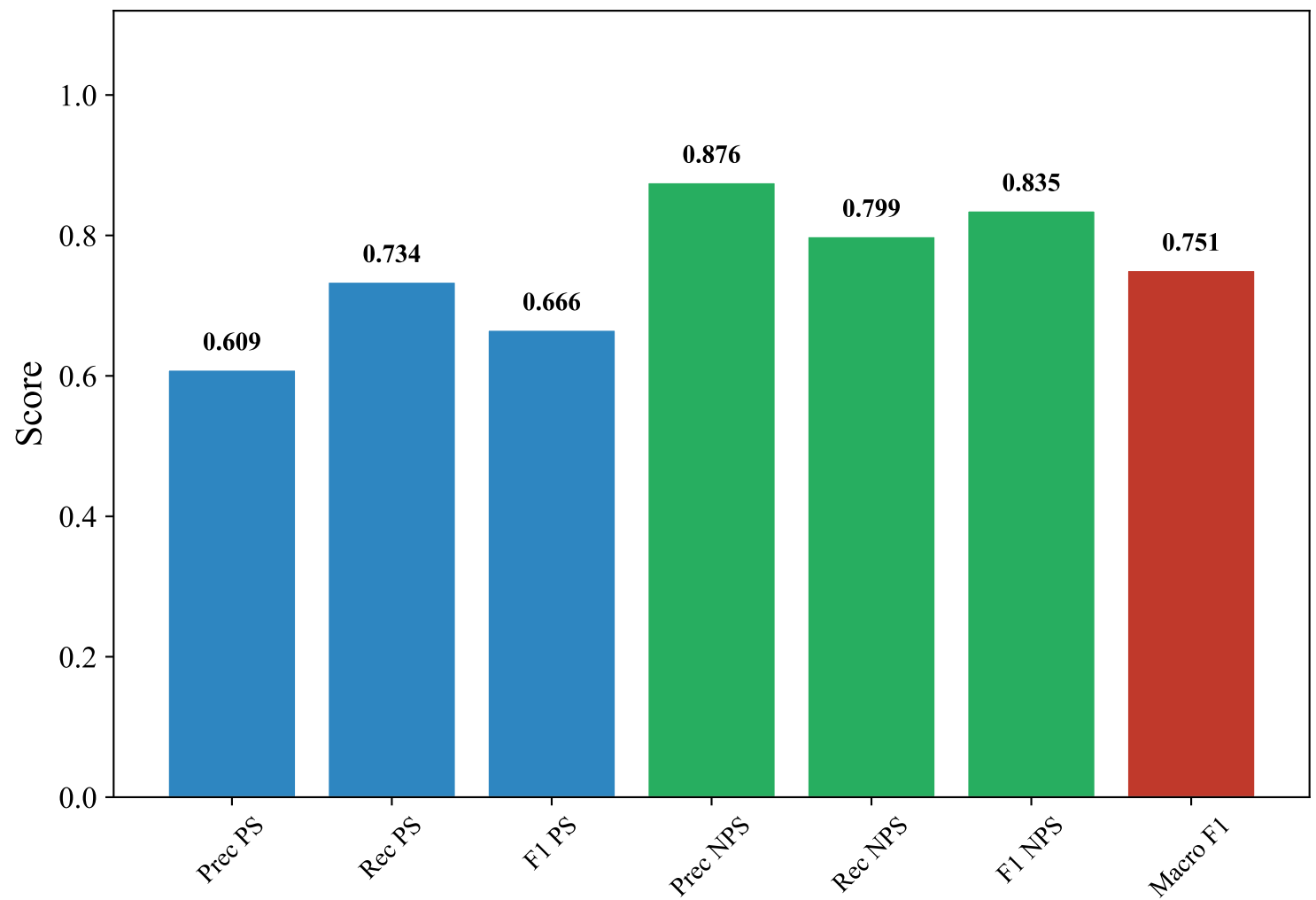
Classification Metrics — ENGLISH_MANUAL (paraphrase-multilingual-mpnet-base-v2, SVM)
