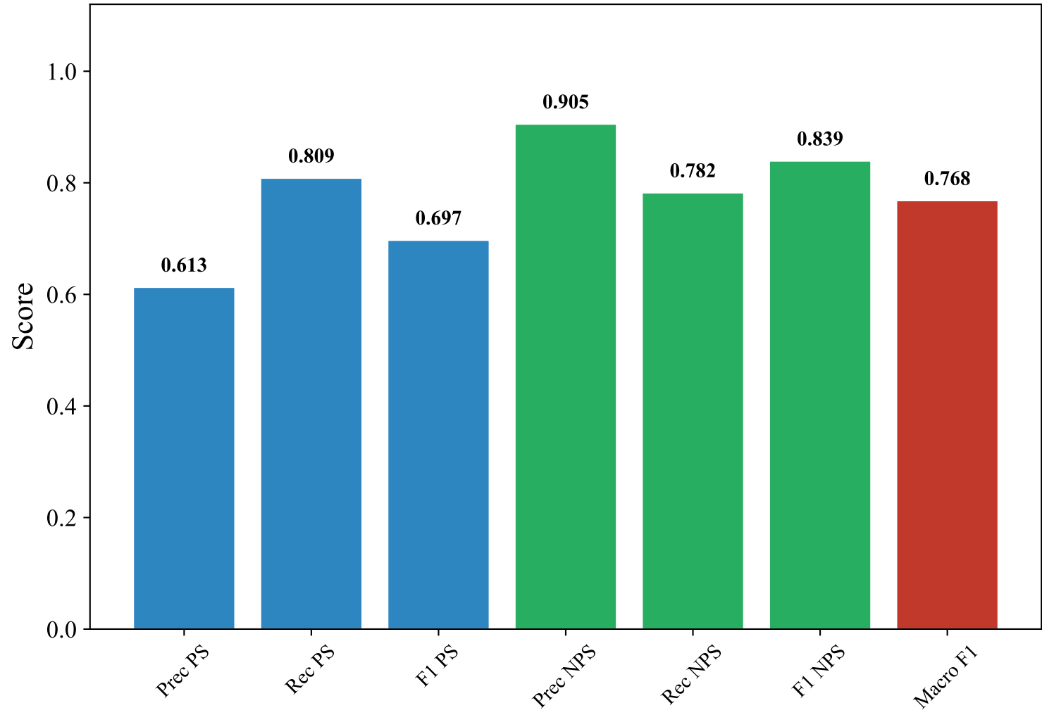
Classification Metrics — ENGLISH_MANUAL (paraphrase-multilingual-mpnet-base-v2, Voting_Ensemble)
