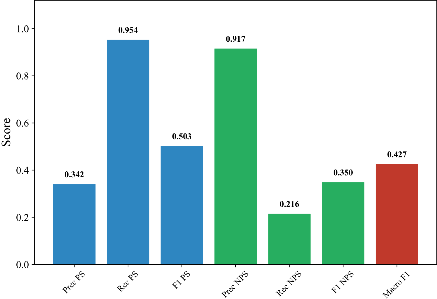
Classification Metrics — ENGLISH_MANUAL (snowflake-arctic-embed-l-v2.0, Random_Forest_Optimized)
