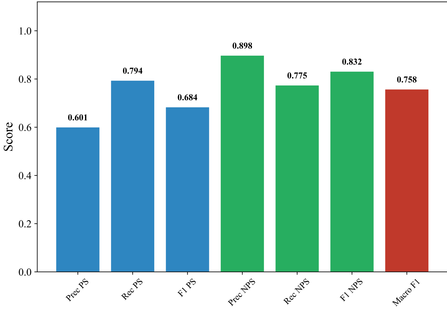
Classification Metrics — ENGLISH_MANUAL (xlm-roberta-base, LightGBM)
