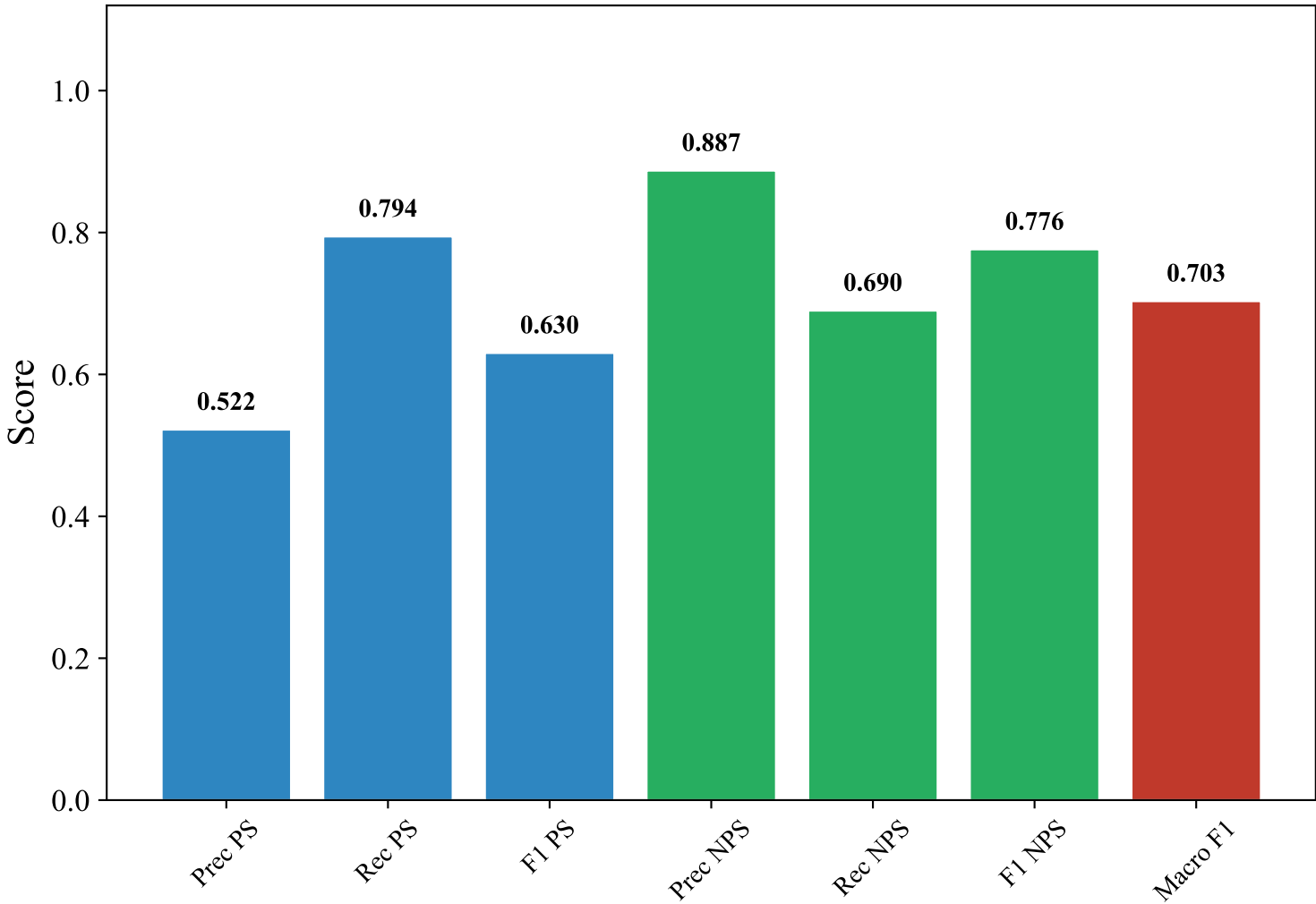
Classification Metrics — ENGLISH_MANUAL (xlm-roberta-base, Random_Forest)
