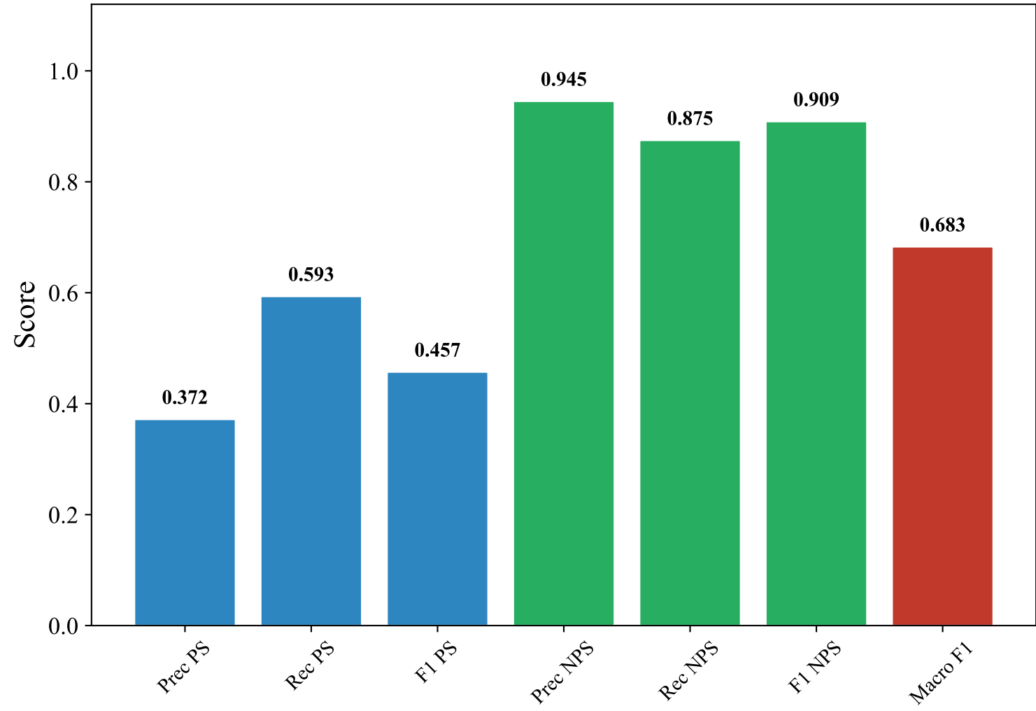
Classification Metrics — GERMAN_MANUAL (efederici/e5-base-multilingual-4096, LightGBM_Optimized)
