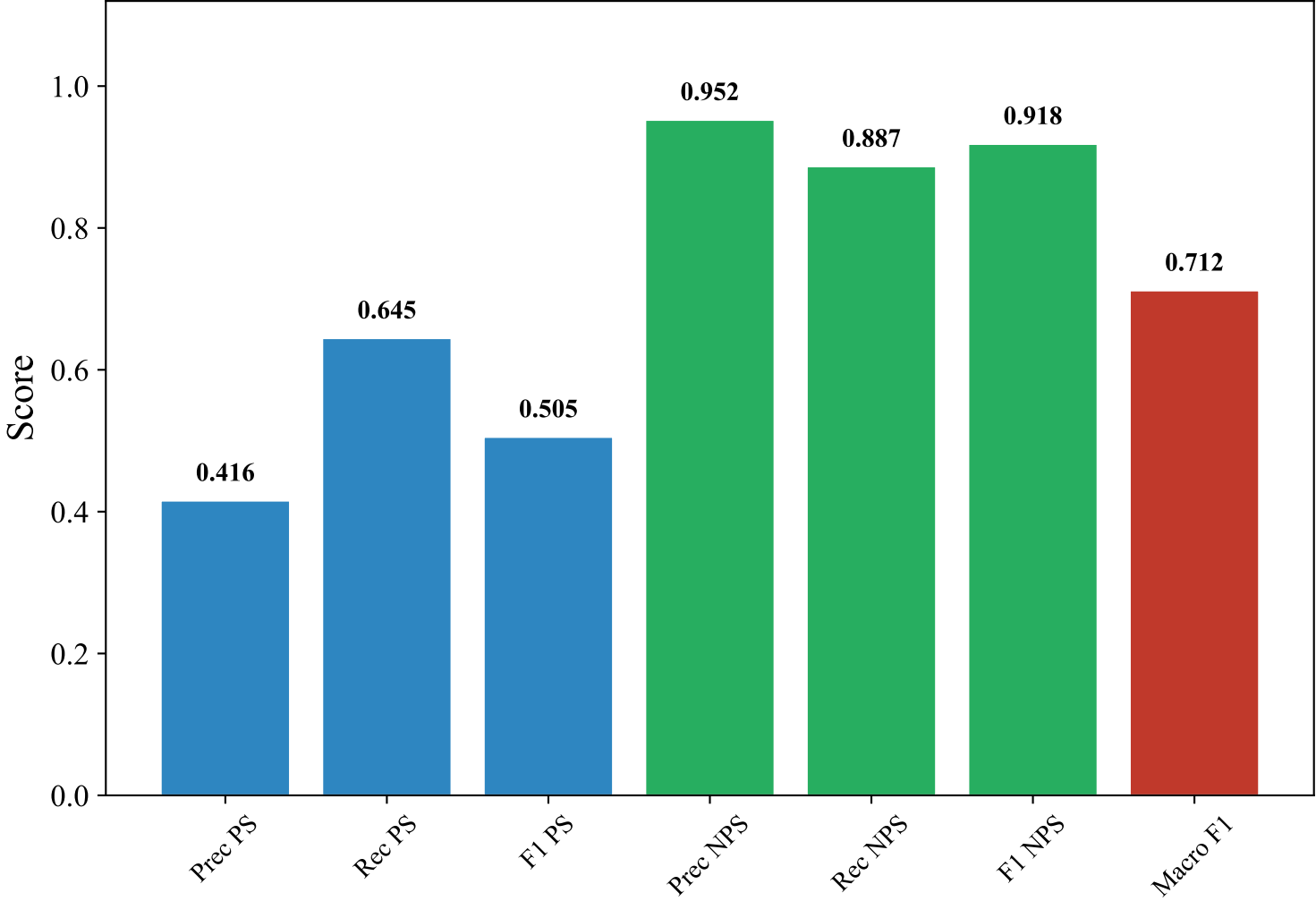
Classification Metrics — GERMAN_MANUAL (intfloat/multilingual-e5-large-instruct, LightGBM_Optimized)
