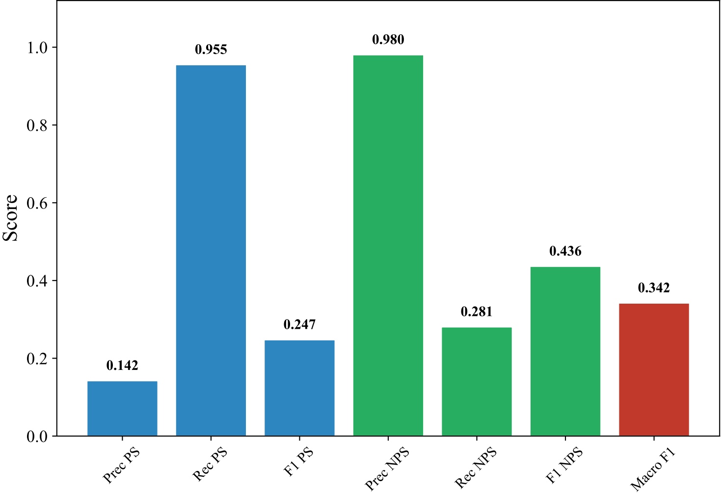
Classification Metrics — GERMAN_MANUAL (intfloat/multilingual-e5-large-instruct, Random_Forest_Optimized)
